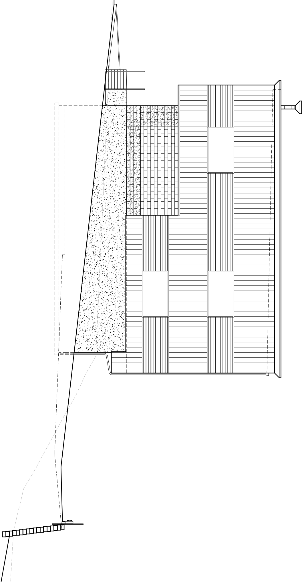
EAST ELEVATION SCALE: 3/16" = 1'-0"
